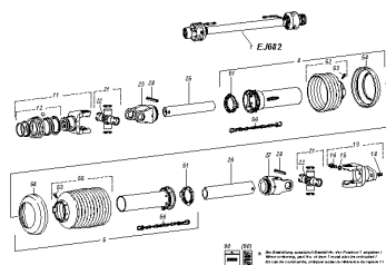
ETB-0000005707, Gelenkwelle EJ682 - W 100 E 810 mm, 1 3/8 Zoll, 6teilig
